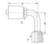
Female FOR-SEAL® Swivel Long Drop 90° Tube Elbow
